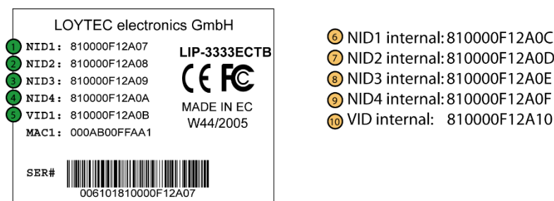
Figure 22: Example of internal NID order on LIP-xxxxECTB.
