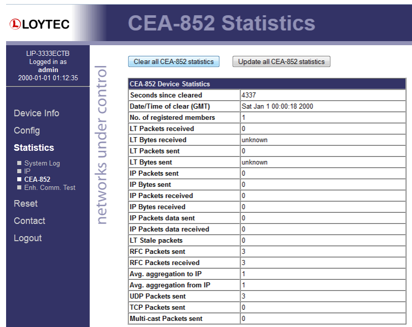
Figure 82: Part of the CEA-852 Statistics Page.
