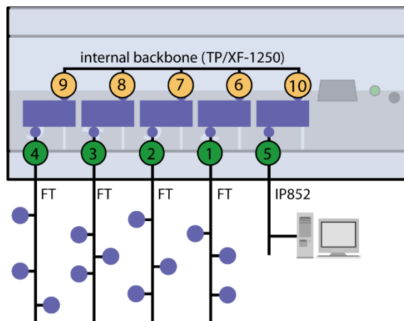
Figure 21: Internal assignment of NIDs on LIP-xxxxECTB.
