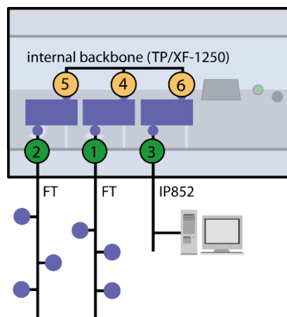
Figure 19: Internal assignment of NIDs on LIP-xxECTB.
