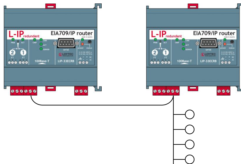
Figure 10: L-IP Redundant in Twin Router mode without Bus Loop Monitoring
