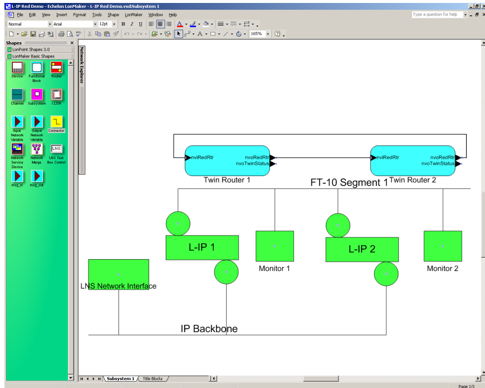
Figure 18: A pair of L IP Redundant devices configured for twin router operation
