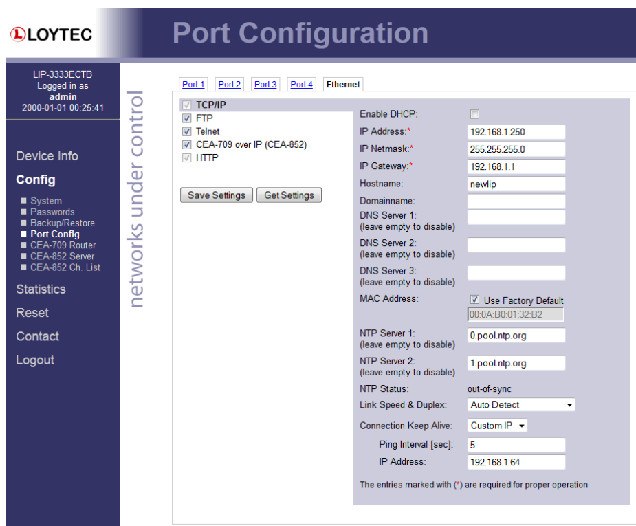
Figure 58: IP Configuration Page.
