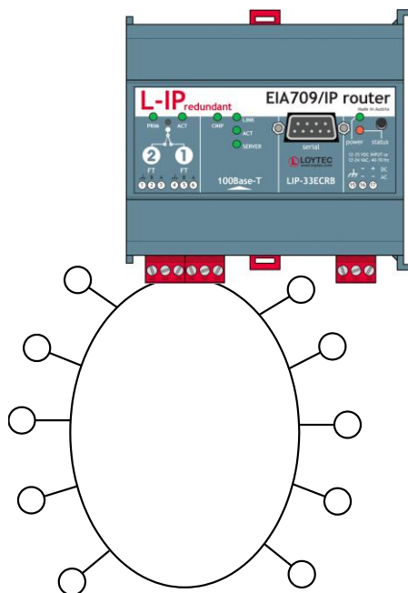
Figure 8: L-IP Redundant Standalone with Bus Loop Monitoring
