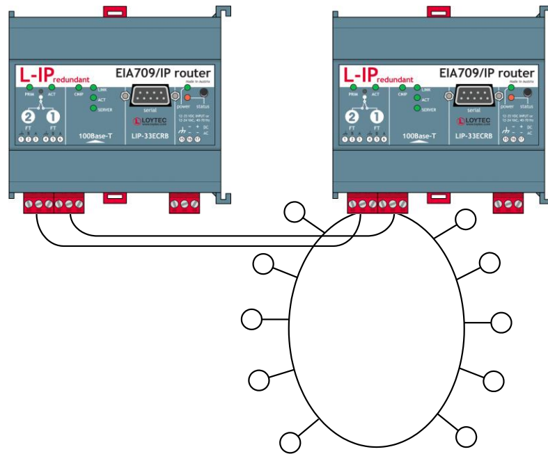
Figure 9: L-IP Redundant in Twin Router mode with Bus Loop Monitoring
